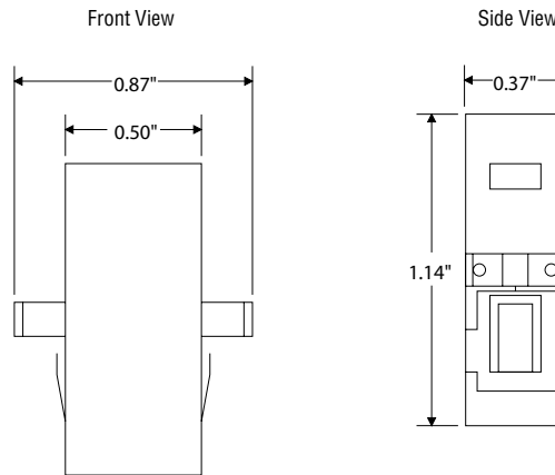
MT-RJ Adapter
